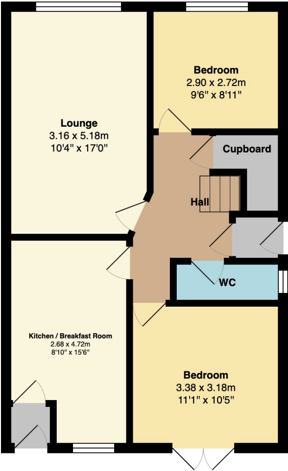
Ground Floor Area: 62.6 m 2 ... 674 ft 2
